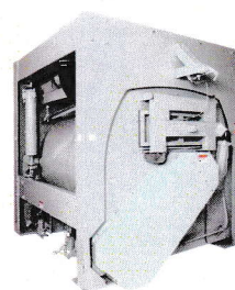
Automatic washer-extractor for mattress cleaning MTE-6
